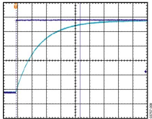
Figure 22. Turn-On Time – C x , C y = 0.1 µF, Time Scale = 2 ms/div
