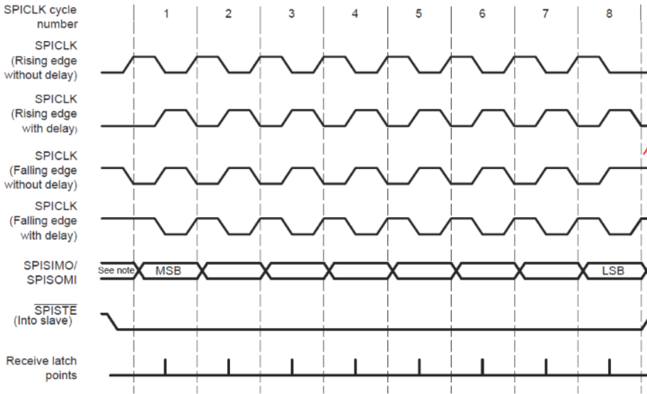
Figure 18-7. SPICLK Signal Options
