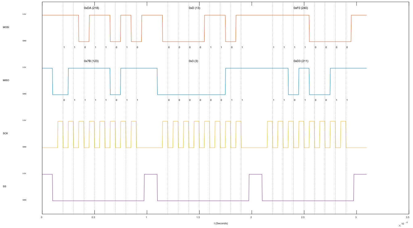
SPI Timing Diagram (MSB First) CLK POLARITY=0 and PHASE=0
