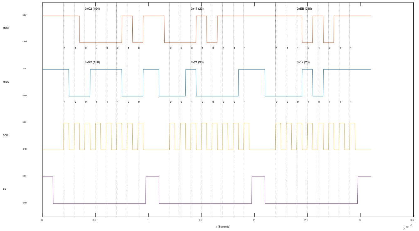
SPI Timing Diagram (MSB First) CLK POLARITY=0 and PHASE=1
